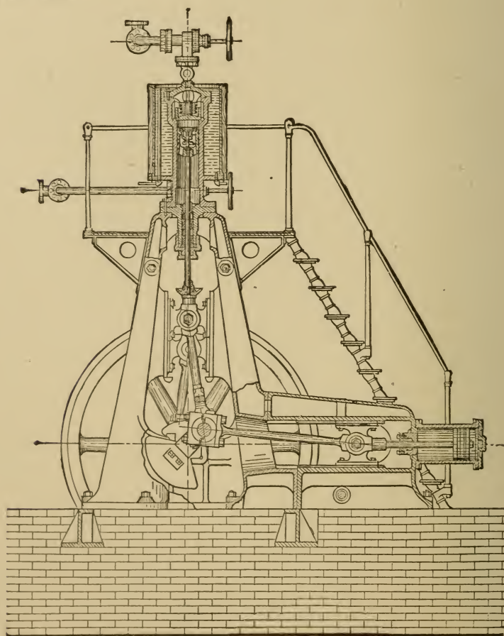
Fig. 127 ICE-MAKING MACHINE.
